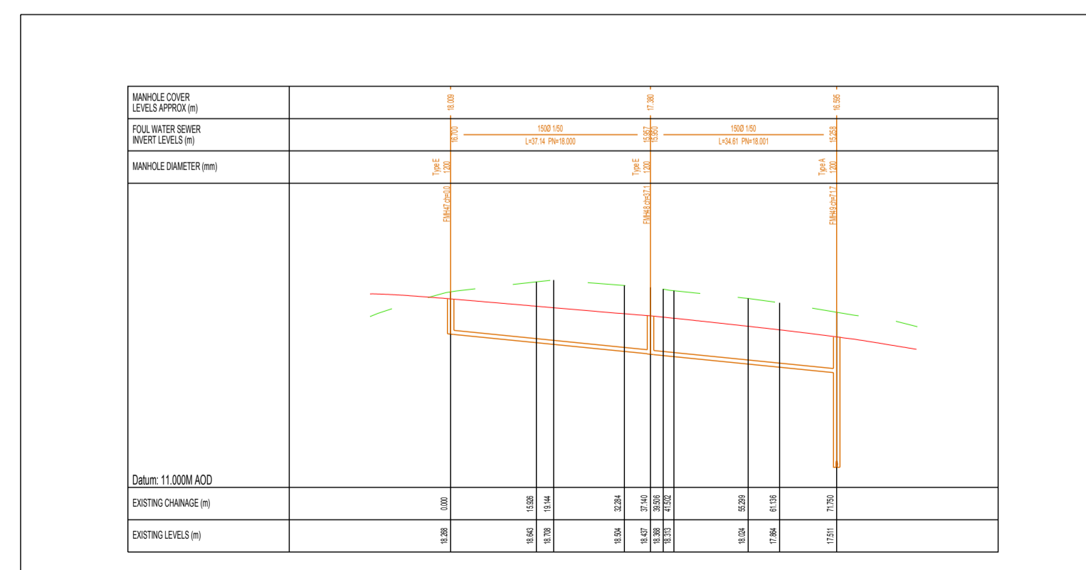
09 Foul Drainage Long Sect 128 SCALE 1:1000
