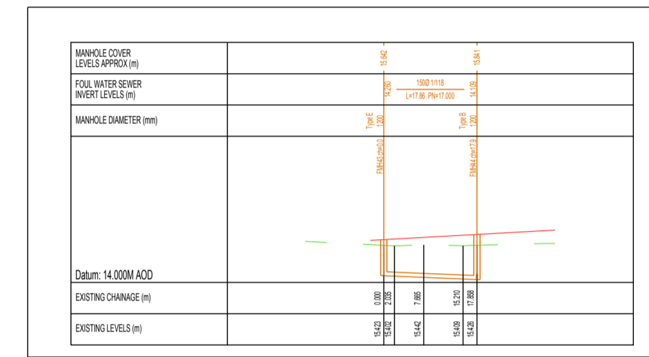
06 Foul Drainage Long Sect 128 SCALE 1:1000
