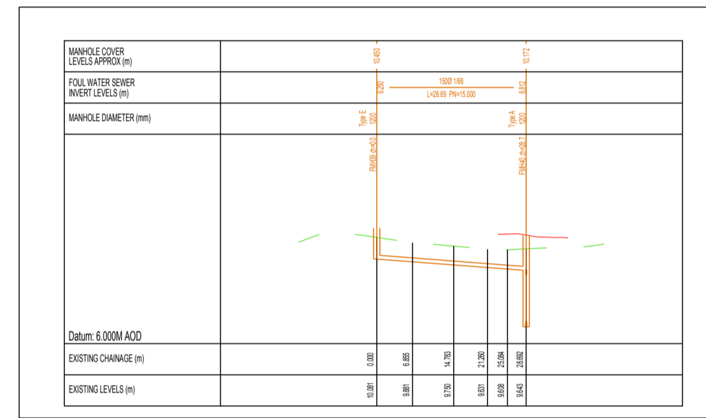
05 Foul Drainage Long Sect 128 SCALE 1:1000
