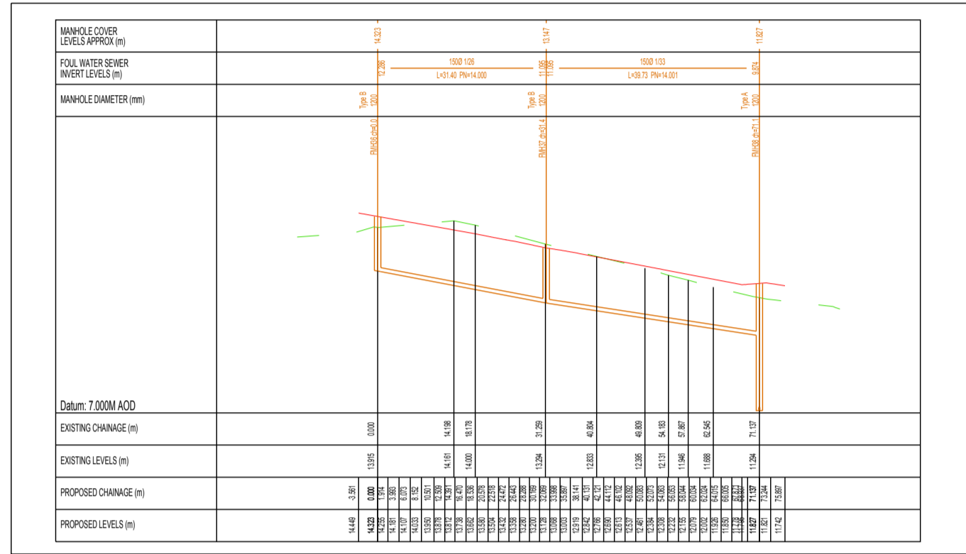
04 Foul Drainage Long Sect 128 SCALE 1:1000
