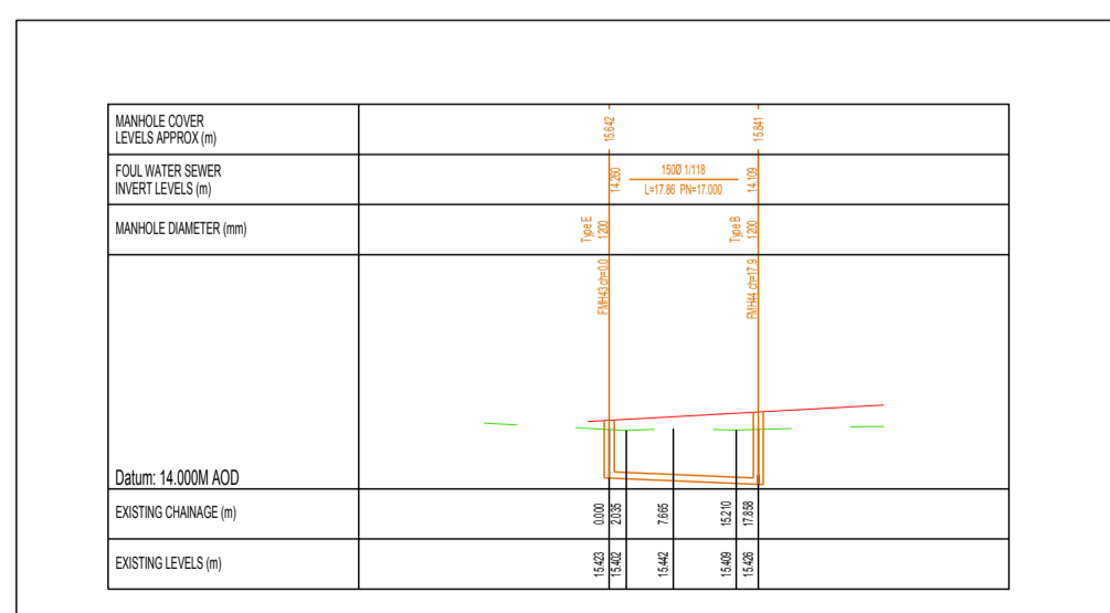
08 Foul Drainage Long Sect 128 SCALE 1:1000
