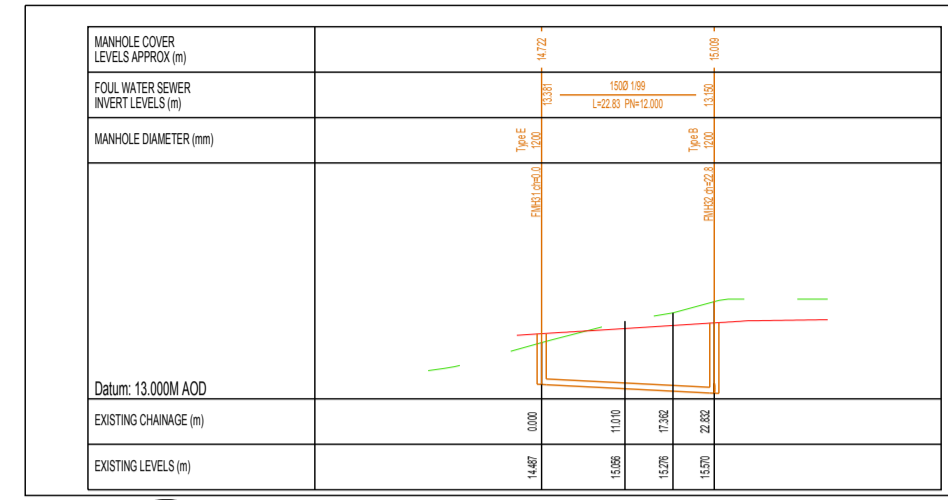
02 Foul Drainage Long Sect 128 SCALE 1:1000
